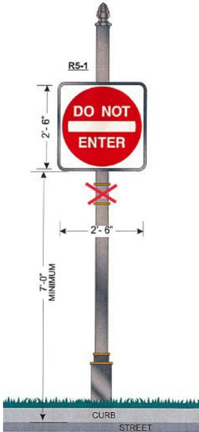
Figure 3.4-E– Type E - 5"x5" Plain 12'-0" High Post (No mid-height collars, No "W")
